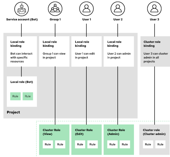
Figure 3: RBAC with Red Hat OpenShift Projects
